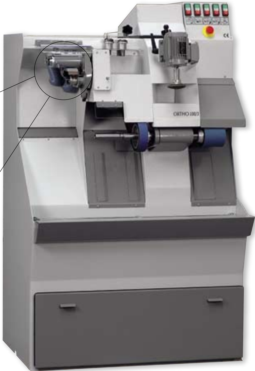
Zwillingsfräsanlage / twin trimming system
